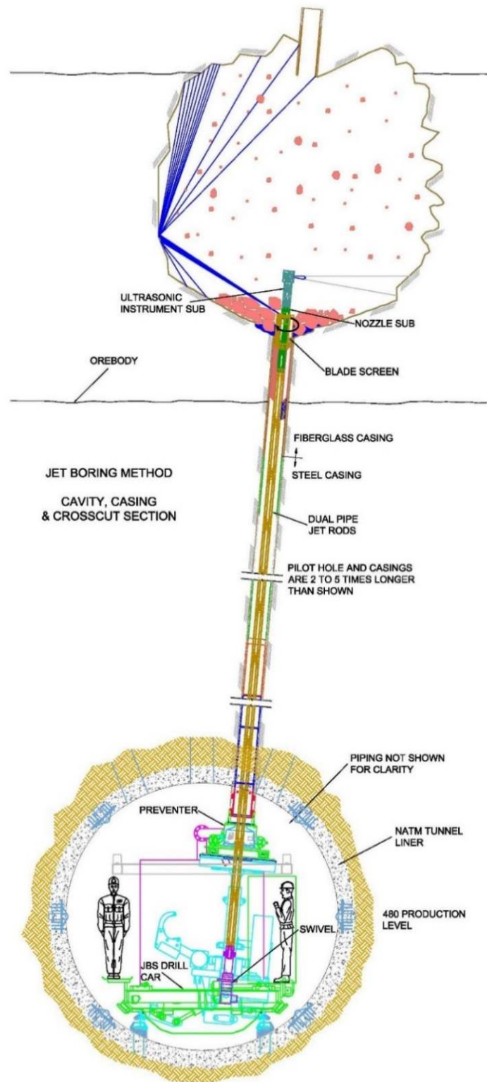
FIGURE 16-8: SCHEMATIC VERTICAL SECTION OF THE JBS MINING METHOD
