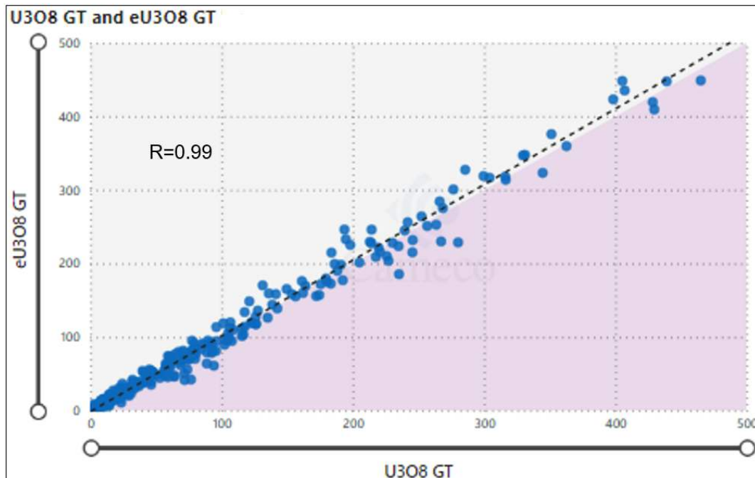
FIGURE 11-1: GT COMPARISON OF \text{eU}_3\text{O}_8 CORRELATION AGAINST CHEMICAL ASSAY
