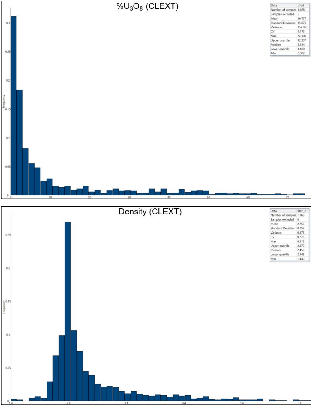
FIGURE 14-8: HISTOGRAM AND SUMMARY STATISTICS OF ALL CLEXT %U 3 O 8 AND DENSITY COMPOSITES
