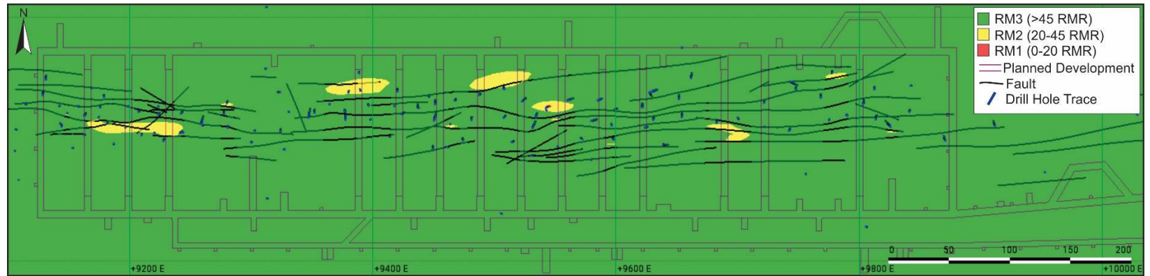
FIGURE 16-2: GEOTECHNICAL DOMAINS OF THE 480L OF CLEXT WITH INTERPRETED FAULT ZONES
