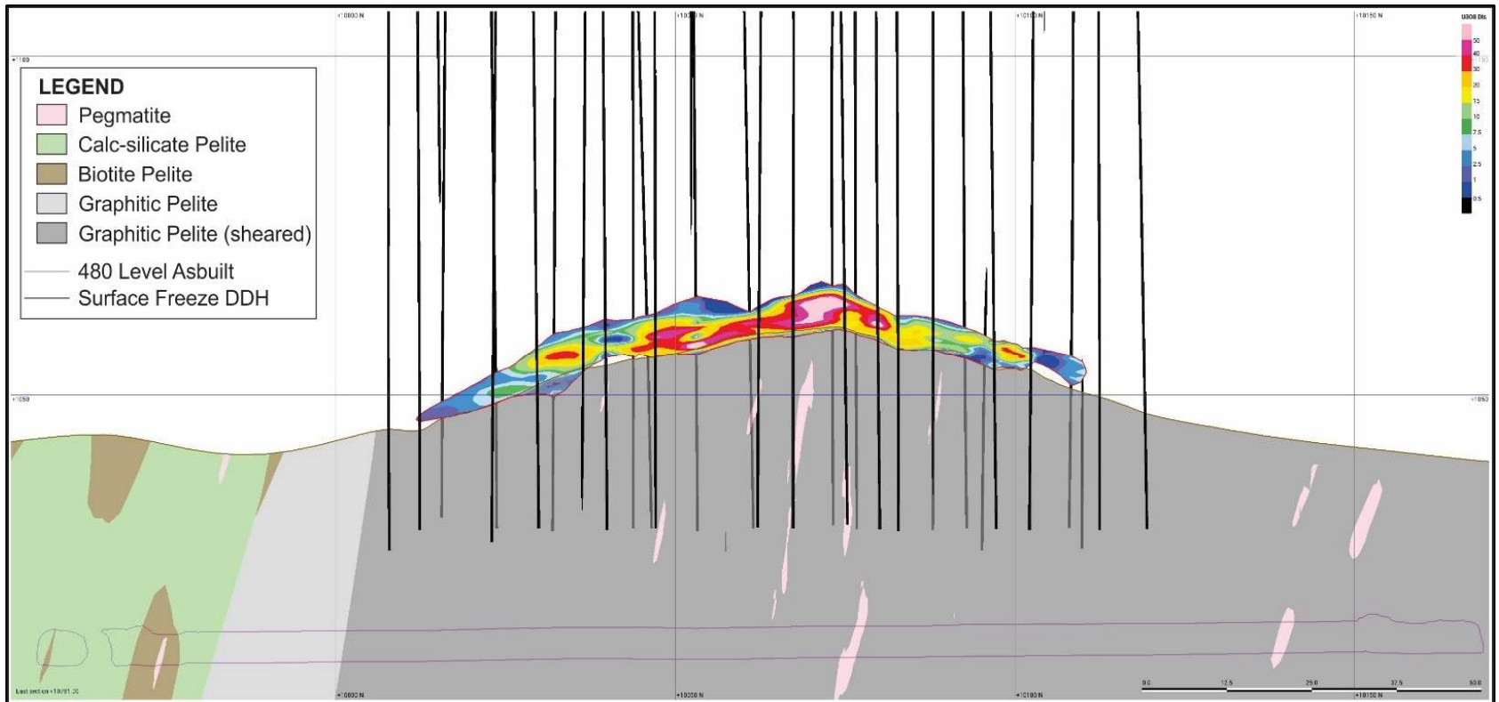
FIGURE 10-3: CL MAIN GEOLOGICAL CROSS SECTION AT 10781E – LOOKING WEST ( \pm 3 m)
