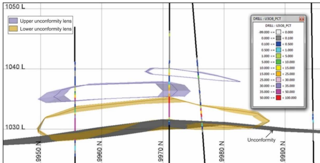
FIGURE 14-6: SECTION 9170E ( \pm 8 m) SHOWING LENSES AND DRILL COMPOSITES - LOOKING WEST
