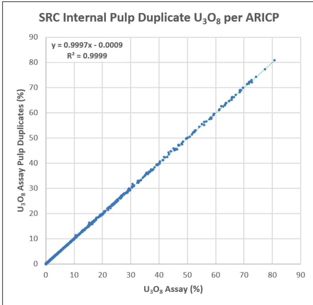
FIGURE 11-3: CIGAR LAKE (CL MAIN AND CLEXT) PULP DUPLICATE AR-ICP RESULTS
