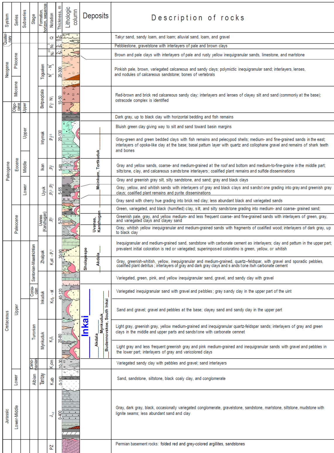
Figure 7-3: Schematic Stratigraphic Column for the Chu-Sarysu Basin
